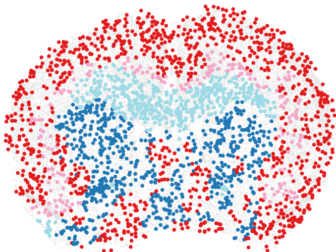
STAMP
